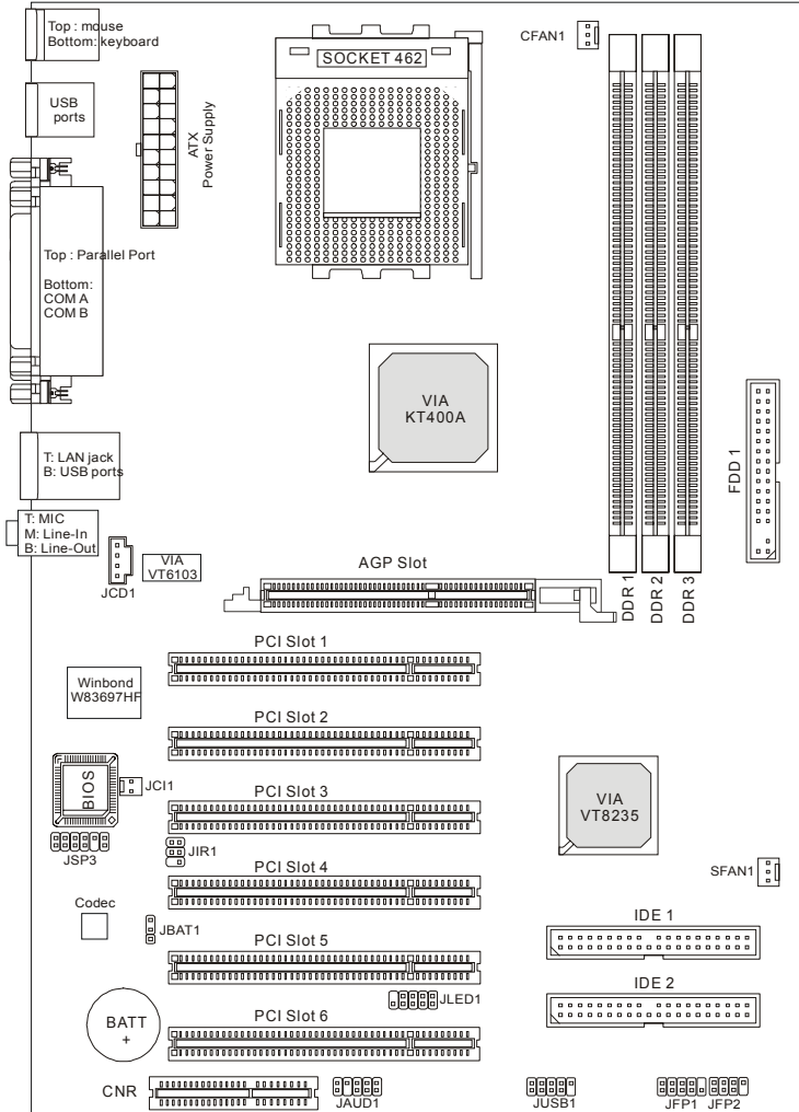
MS-6712 v1.X ATX Mainboard
