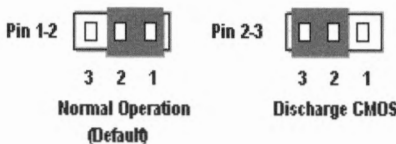
Figure 2-8. CCMOS1 jumper setting
