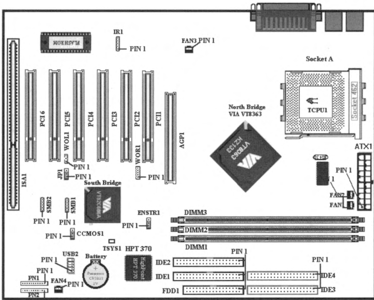
Figure 2-7A. All Connectors and Headers for the KT7-RAID
