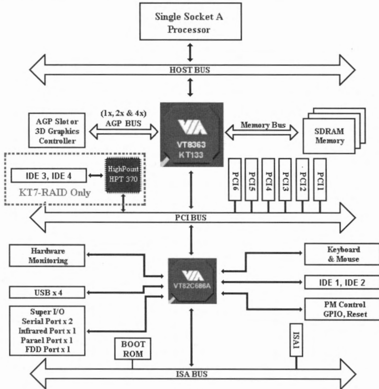
Figure 1-2. System diagram of the KT7/KT7-RAID
