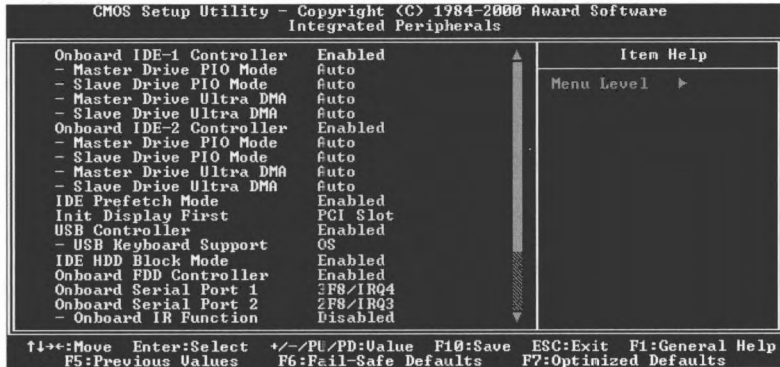
Figure 3-6A. Integrated Peripherals Menu Default Screen (KT7)
