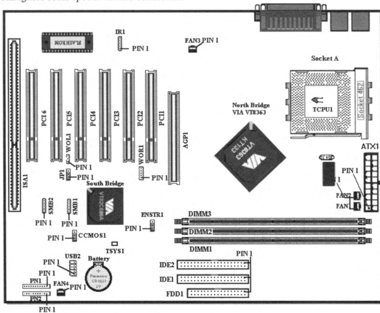
Figure 2-7. All Connectors and Headers for the KT7
