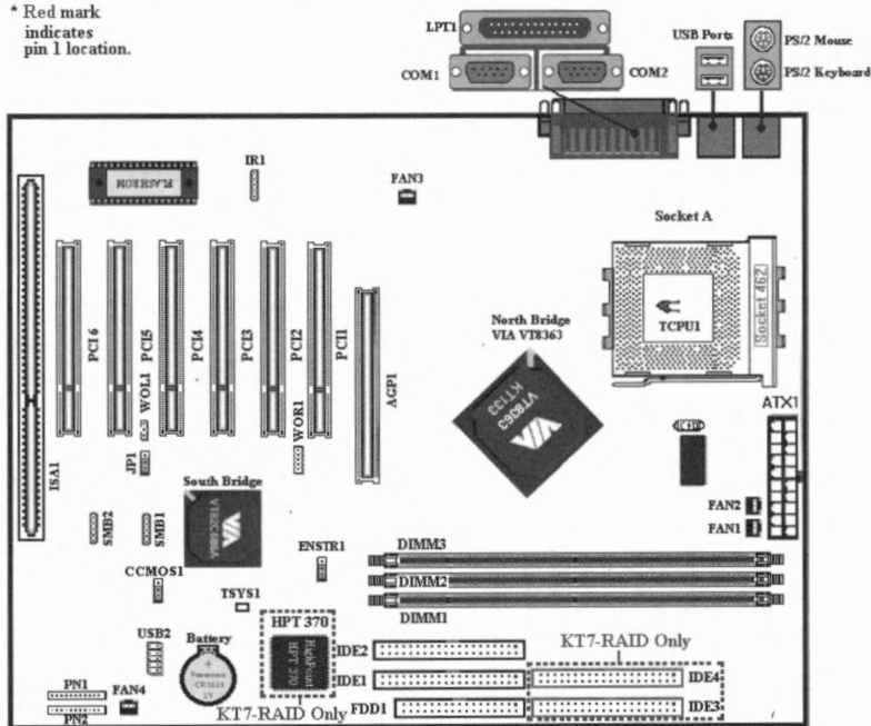
Figure 1-1. KT7/KT7-RAID Motherboard component location
