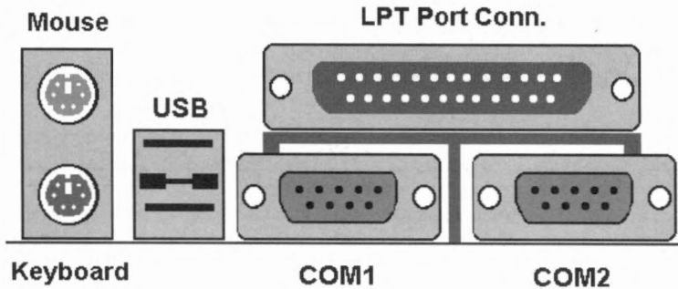
Figure 2-11. KT7/KT7-RAID back panel connectors
