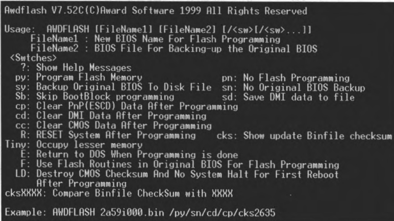
Figure F-3. Award Flash Memory Writer V7.52C Flash Commands Screen
