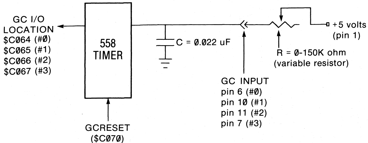
Figure 10-3. Block diagram of game controller circuitry.
