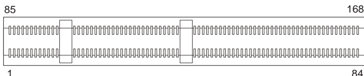
Figure 27 (Page 1 of 3). System Memory Connector Pin Assignments
