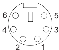
Figure 40. Mouse and Keyboard Port Connector Pin Assignments
